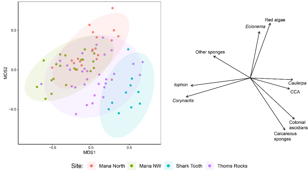
Figure 6. Multidimensional scaling (MDS) plot of benthic sessile communities for a combination of site (represented by symbol colour) with overlaid vector of species contribution to spatial separation.
