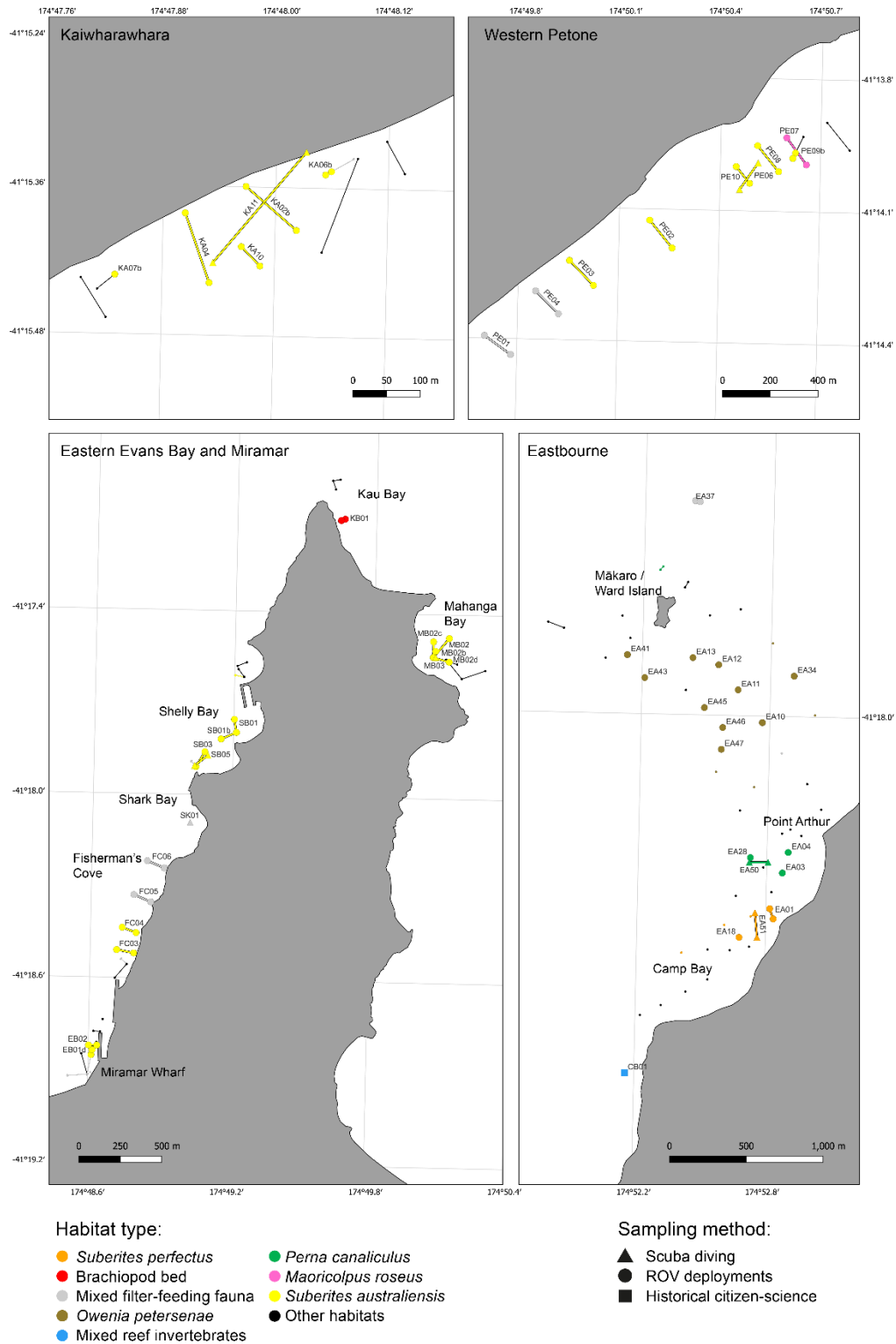
Figure 2. Details of the surveyed stations in Wellington Harbour (WH). Sampling stations with a habitat quality score below 6 (see section 2.3.3) were represented with smaller points. For visual clarity, station names are only reported for stations scoring 6 or above.
